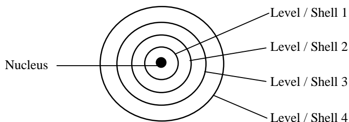
Energy Levels or Shells
